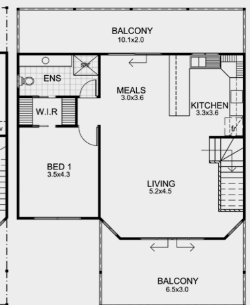
UPPER LEVEL
